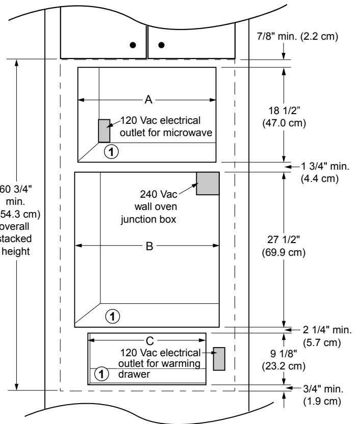
CUTOUT DIMENSIONS DCM24 SHOWN
