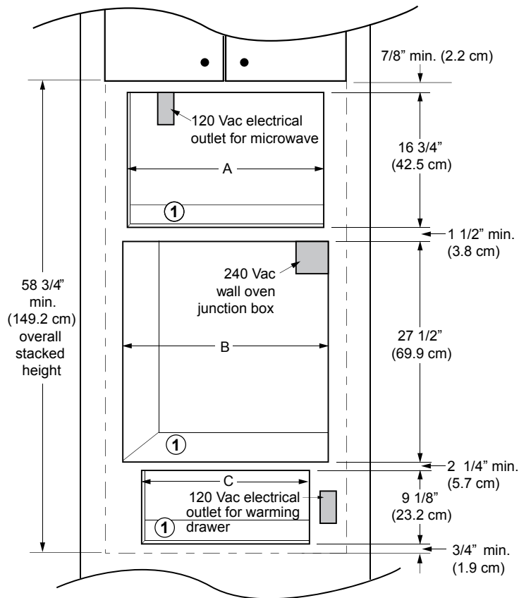
CUTOUT DIMENSIONS DMT2420/DMW2420 SHOWN
